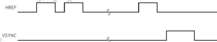
figure 6-2 compression mode 2 timing
